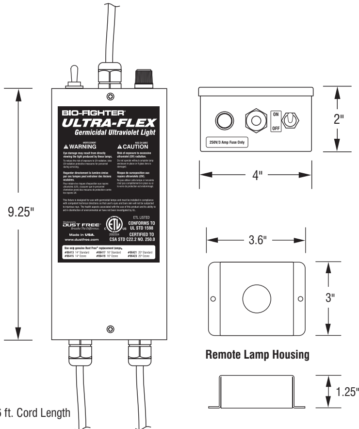
Fig. 1 Dimensions of single and dual bulb Ultra-Flex.
