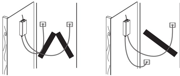
Ultra-Flex mounted on wall near air handler. Remote lamp cords allow the Ultra-Flex to be mounted anywhere within 6 feet of the air handling unit.
