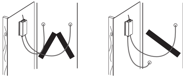
Aqua-Seal mounted on wall near air handler. Remote lamp cords allow the Aqua-Seal to be mounted anywhere within 6 feet of the air handling unit.
