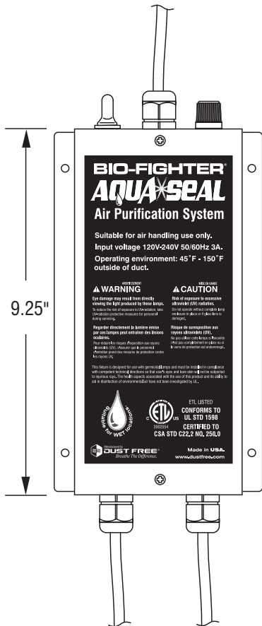
Fig. 1 Dimensions of single and dual bulb Aqua-Seals.
